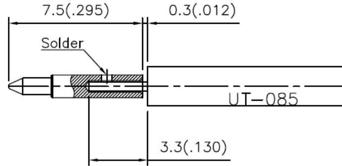
CENTER CONTACT
